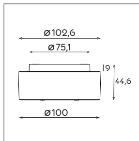
Fig. 2: Canopy (side view)
